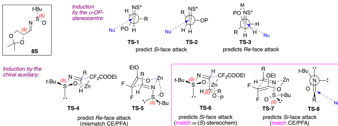
Figure 1. Models to explain the stereoinduction/double diastereodifferentiation.
